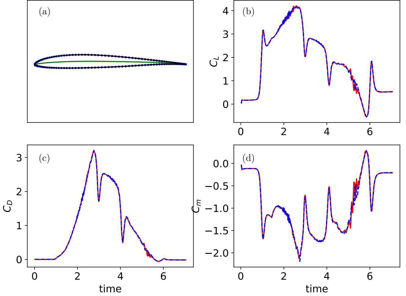
Figure 3: Validation of the LDVM implementation. (a) shows the profile (—), its interpolation (··) and the camber line (—). (b), (c), (d) show respectively C_L , C_D , C_m obtained with the fortran implementation (---) and our python implementation (—).
